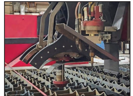
KINETIC BEVEL CUTTING HEAD & OXY TORCH HEAD
