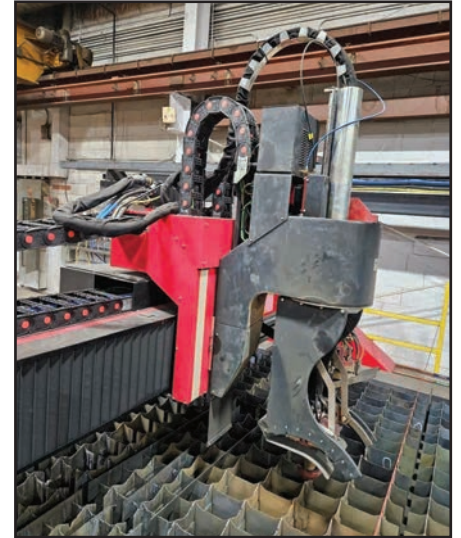
KINETIC BEVEL CUTTING HEAD
